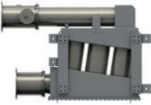
Cat C18 and C32 CEM Air-Assist, U.S. EPA Tier 4 and IMO Tier III U-Flow or Z-Flow configured
